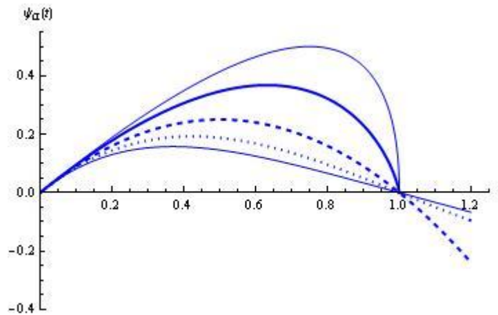
Figure 2 Adjoint power information functions, \alpha = 0.5, 1, 2, 3, 4
