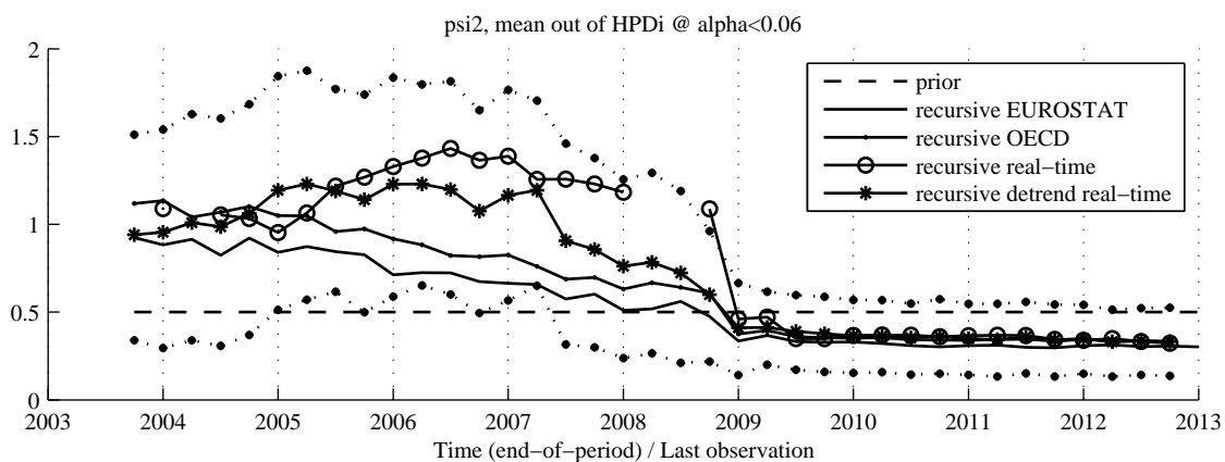
Figure 4 Recursive estimates of the weight on output growth in a domestic Taylor rule
