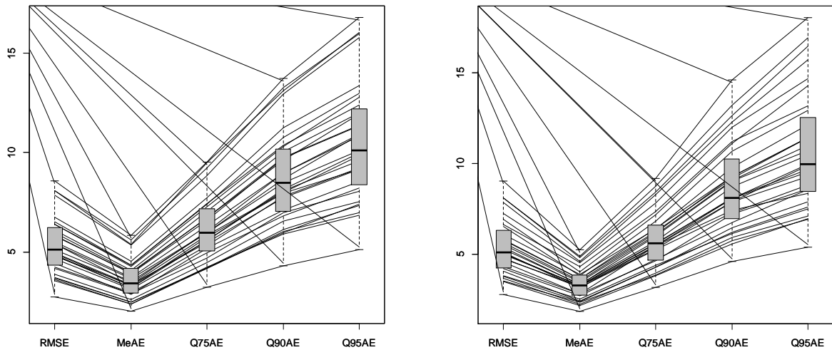
Figure 2 Relative accuracy (in %) of EBLUP for N (on the left) and E (on the right) cases for D=31 domains
