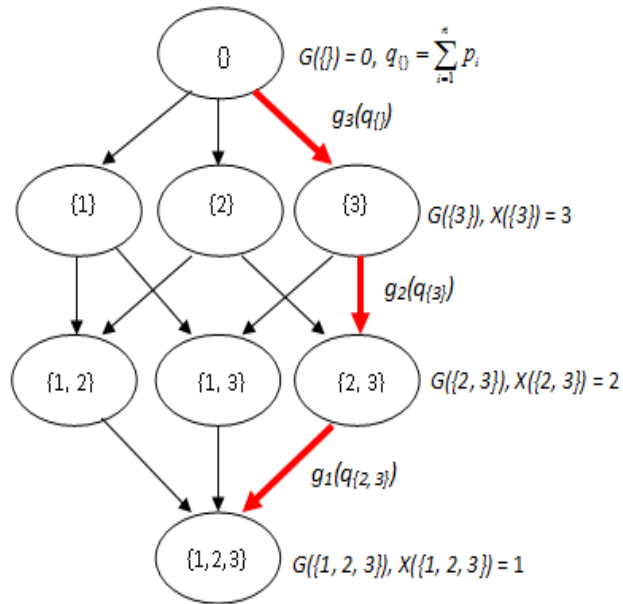
Figure 1 Digraph D
