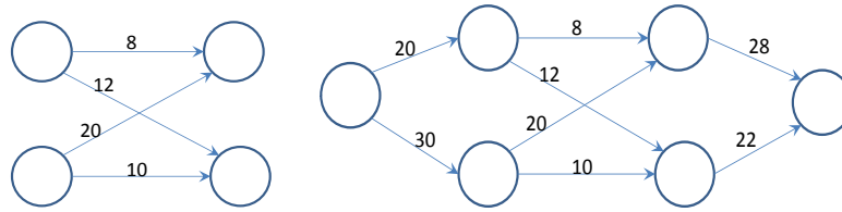
Figure 1 The transformation of the graph with more sources and sinks into the graph with one source and one sink
