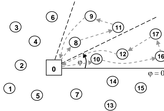
Figure1 Principle of the sweep algorithm
