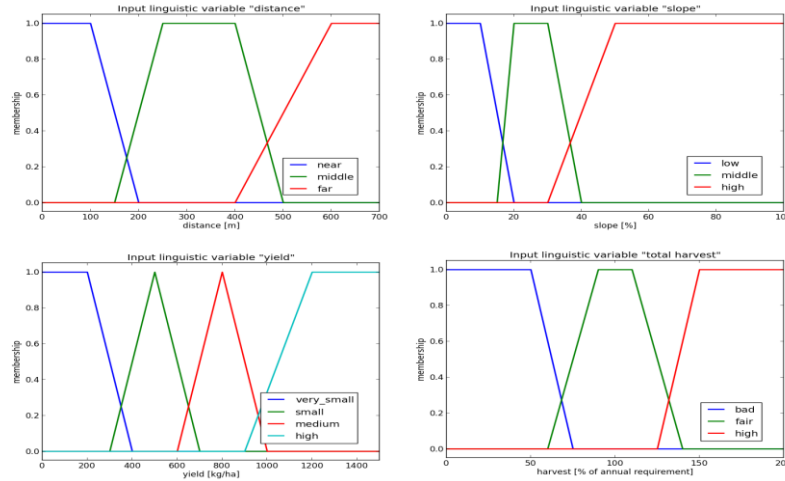
Figure 1 – input variables of the fuzzy inference system
