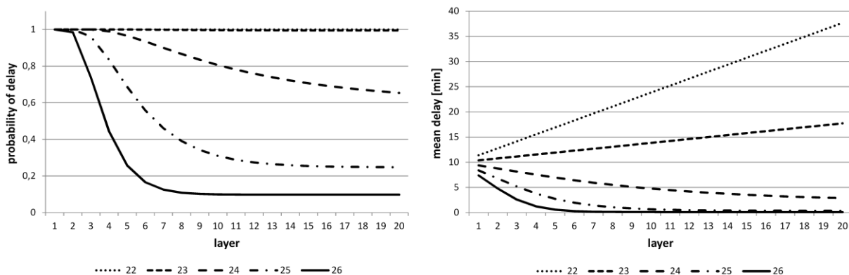
Figure 4 Model behavior in case of unexpected initial delay \delta = 10 minutes
