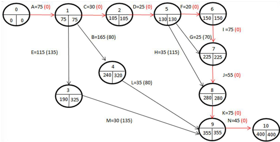
Figure 1 Small-scale project with the indication of a critical path.
