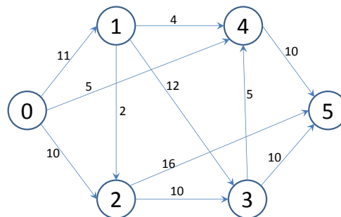
Figure 3 The graph for the numerical experiment
