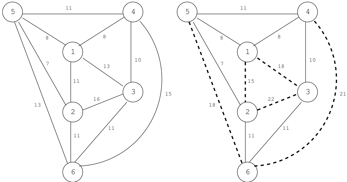
Figure 1 Original and reduced transportation networks
