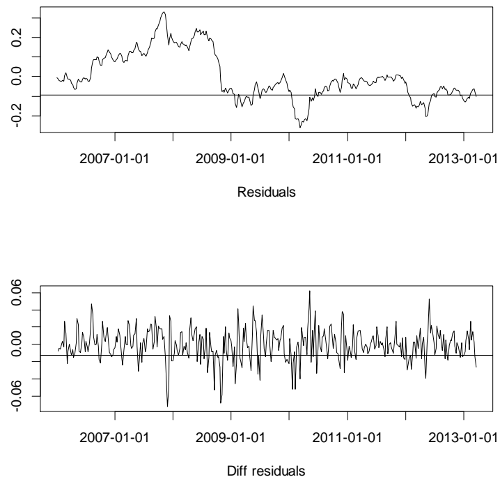
Figure 2 Thresholds values for c.tar and c.mtar models
