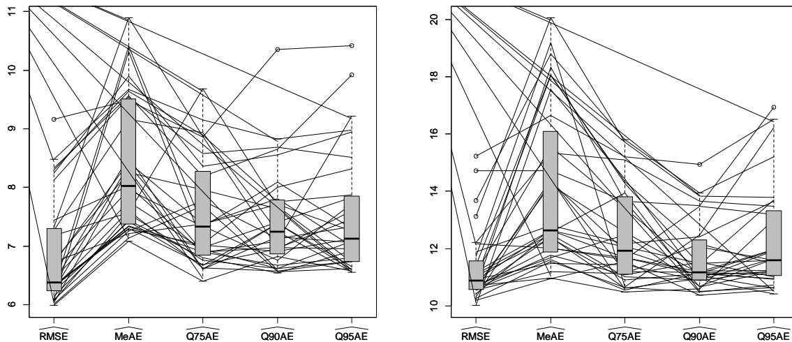
Figure 4 Relative RMSEs (in %) of accuracy estimators of EBLUP for N (on the left) and E (on the right) case D=31 domains
