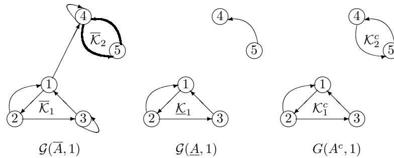
Figure 2: Threshold digraphs
