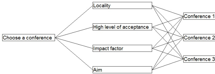
Figure 1 Hierarchy graph
