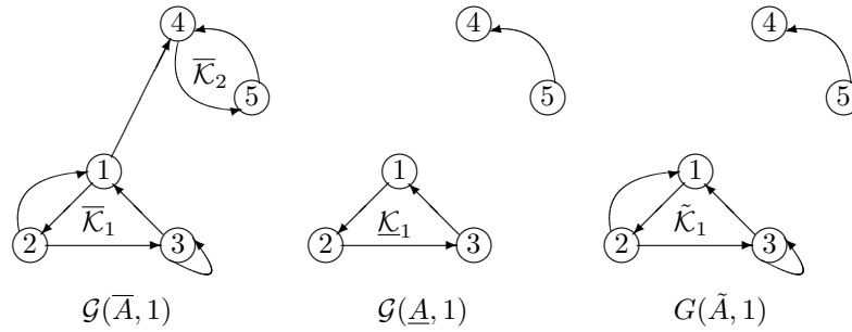
Figure 1: Threshold digraphs
