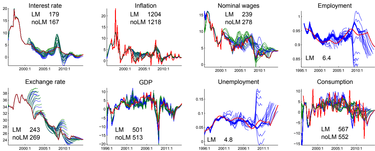
Figure 2 In-sample forecasts
