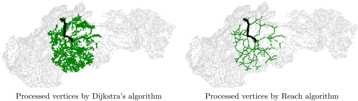
Figure 2: Processed vertices by one direction only algorithm
