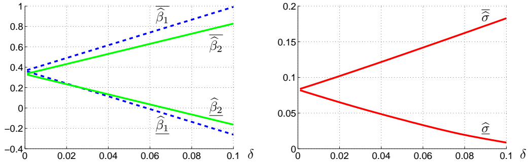
Figure 2 Ranges for \hat{\beta}_1 , \hat{\beta}_2 and \hat{\sigma} with \delta \in [0, 0.1] .
