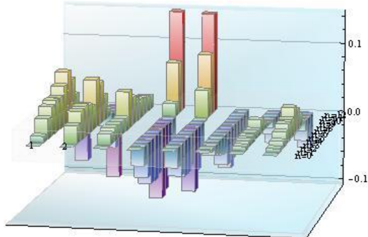
Figure 8 Difference vectors \Delta(t) = p(t) - q(t) at t=2005Q1,\dots,2011Q1 , and 2011Q3, 2012Q1
