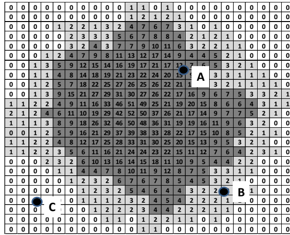
Figure 2 An example of critical region based on cells division.
