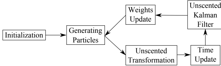
Figure 1 Unscented particle filter
